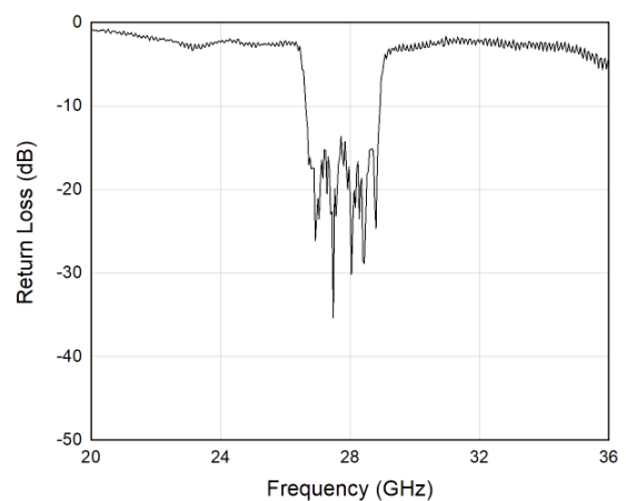
Figure 3. Return Loss
