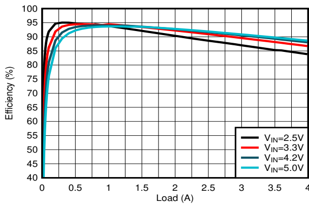
Figure 9-11. Efficiency
