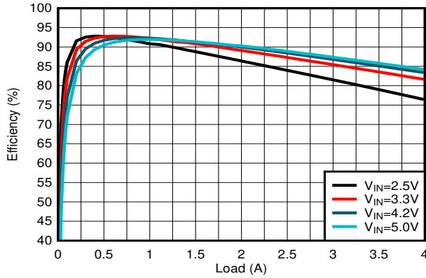
Figure 9-9. PWM Efficiency
