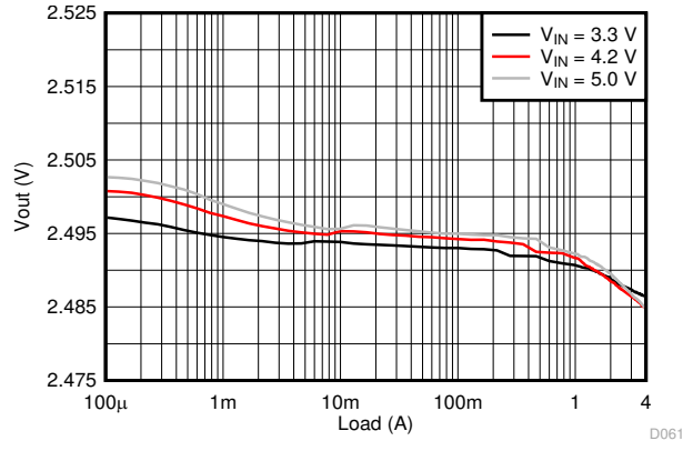
Figure 9-16. Load Regulation
