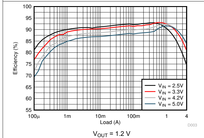
Figure 9-7. Efficiency
