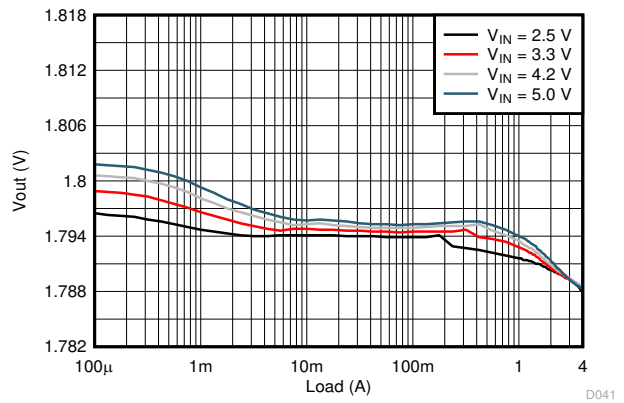
Figure 9-12. Load Regulation
