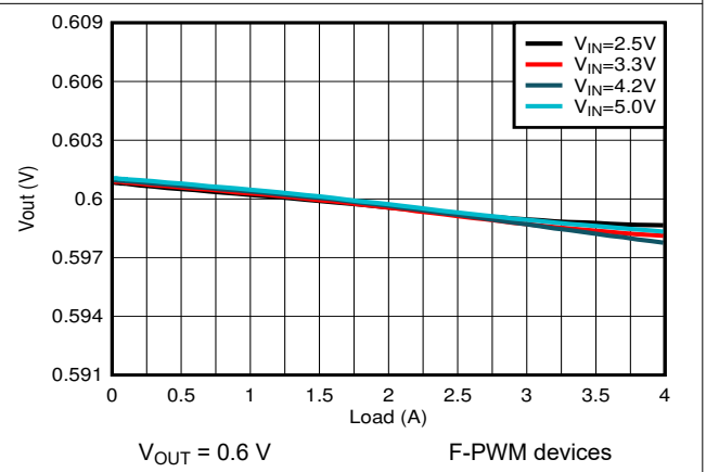
Figure 9-6. Load Regulation
