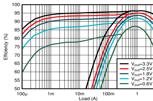
Efficiency at V_{IN} = 5\text{ V}
