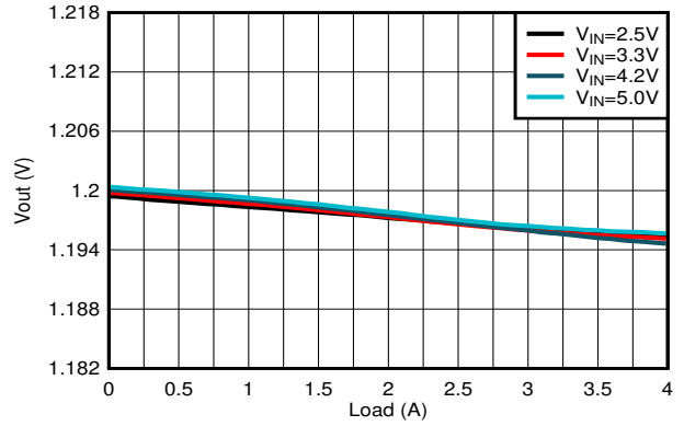
Figure 9-10. Load Regulation
