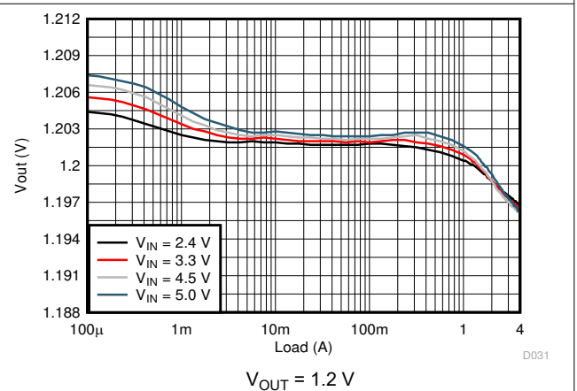
Figure 9-8. Load Regulation
