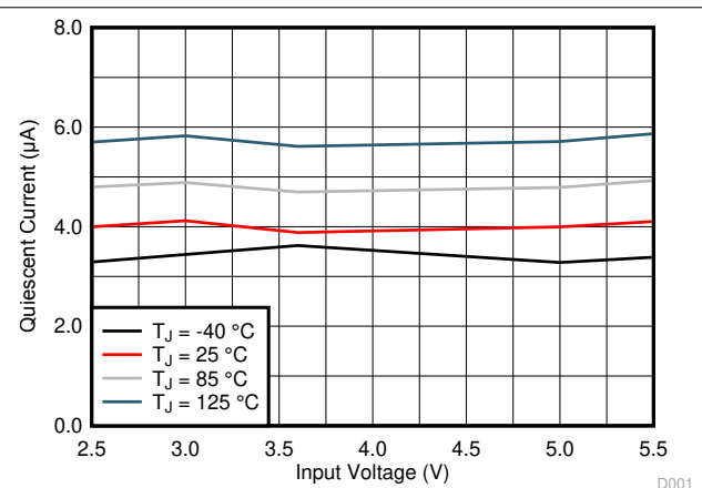
Figure 7-4. Quiescent Current
