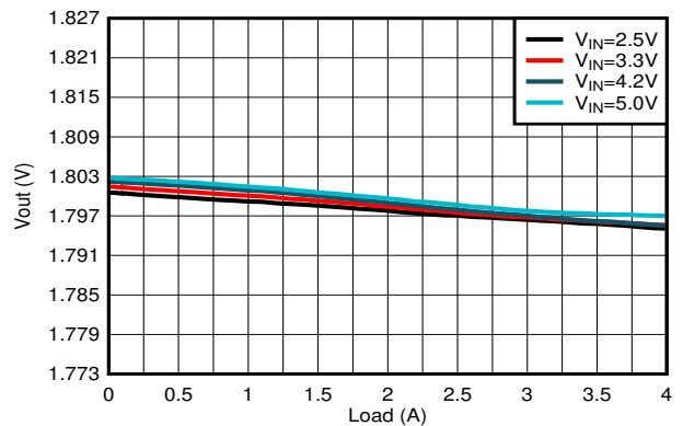
Figure 9-14. Load Regulation
