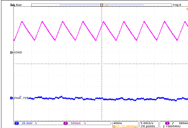
I OUT = 1.0 A TPS62824A/5A/6A/7A
