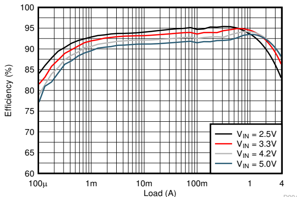
Figure 9-9. PWM Efficiency
